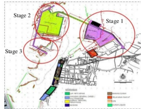
Fig. 2. Soekarno-Hatta port development plan
