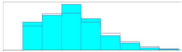
Fig. 6. Ship visits distribution ( Poisson distribution)
