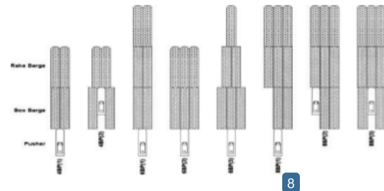
Fig. 8. Container transport with push barge system (Koh King Koh, Hironori Yasukawa, Noritaka, Hirata 2008)
